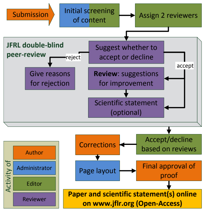
Abridged version of the review flow chart, full version available online
